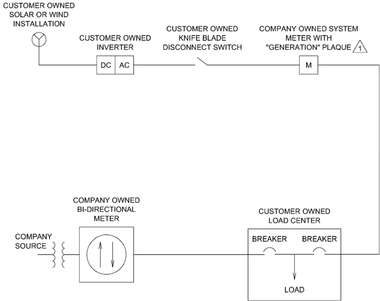
Residential-Customer Owned Generation Schematic Diagram
